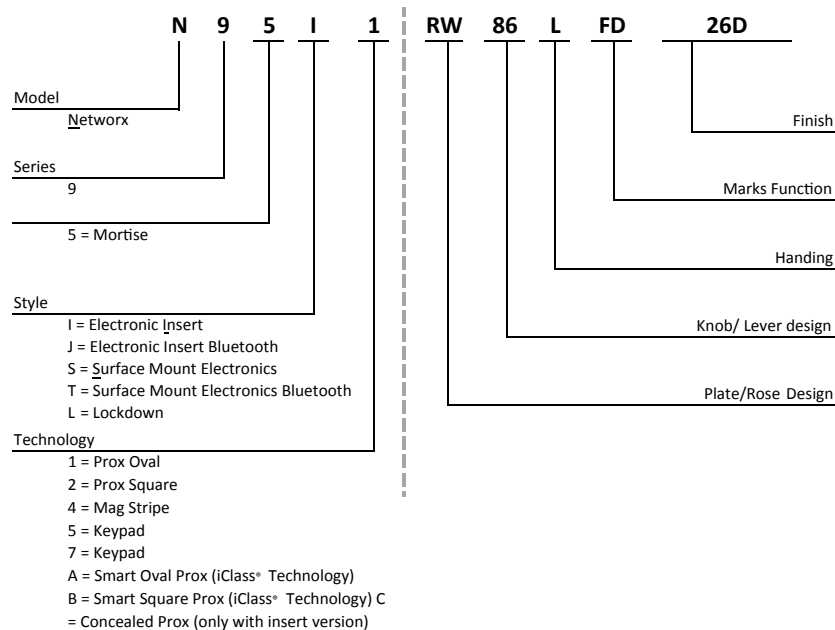
BASE DISTRIBUTION MORTISE MODEL P/N SCHEME
